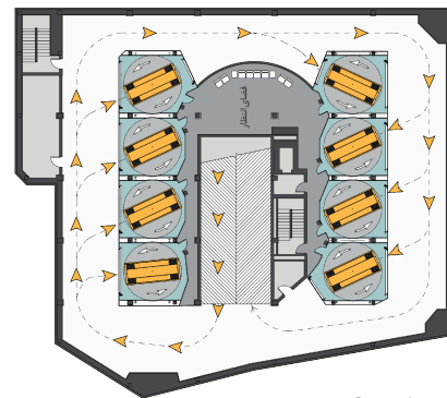
Entrance floor plan Entrance circulation
